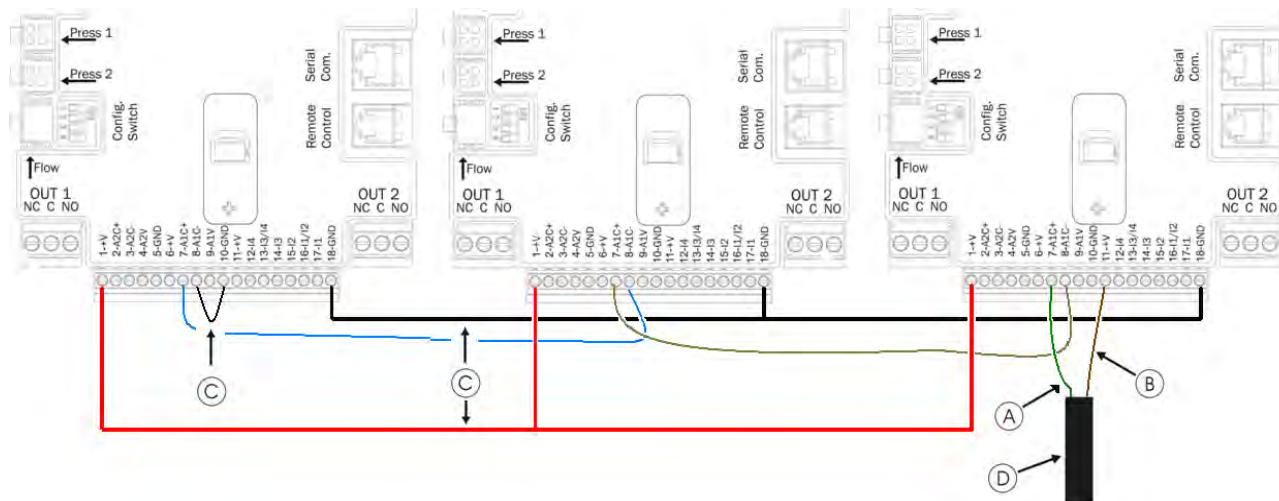
Figure 9: Connection of 4 - 20 mA pressure sensor on a multiple inverter system
