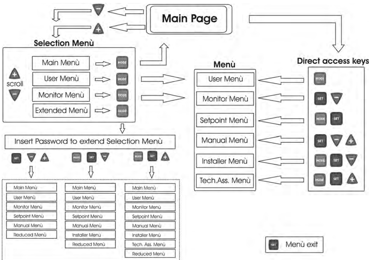
Figure 14: Optional menu access scheme
