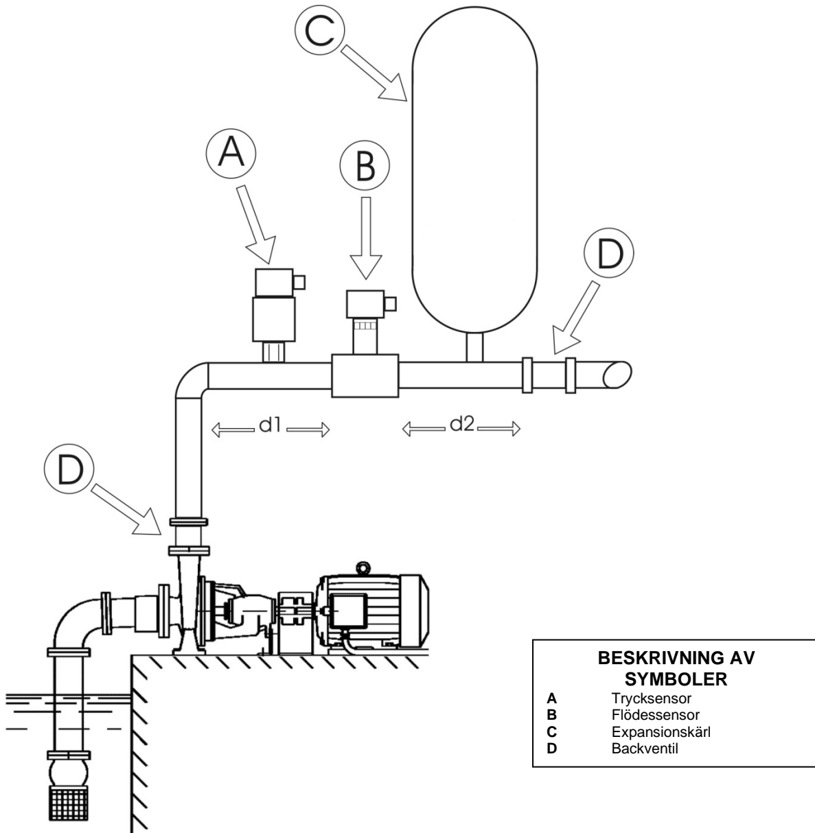
Fig. 6: Hydraulisk installation
