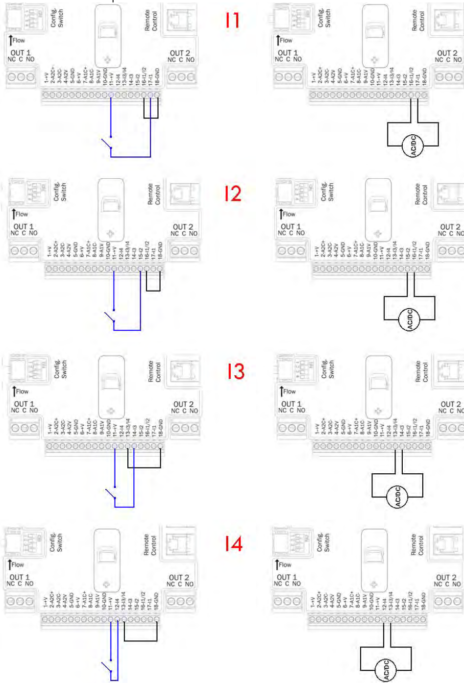
Figure 11: Example of input connections
