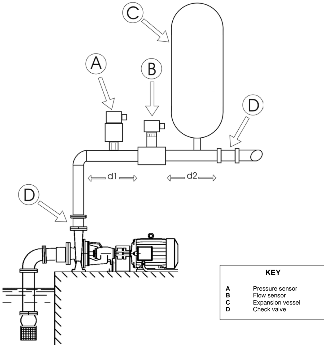
Figure 6: Hydraulic installation
