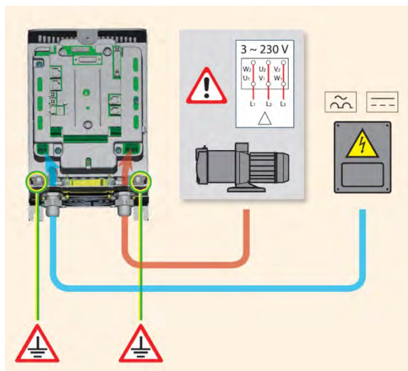
Figure 5: Pump connection PWM 203 - 202 – 201
