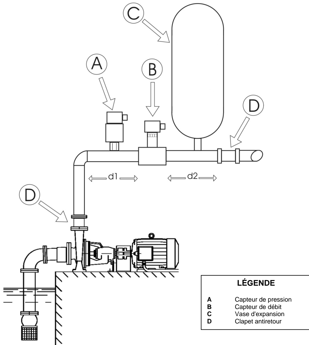
Figure 6: Installation hydraulique
