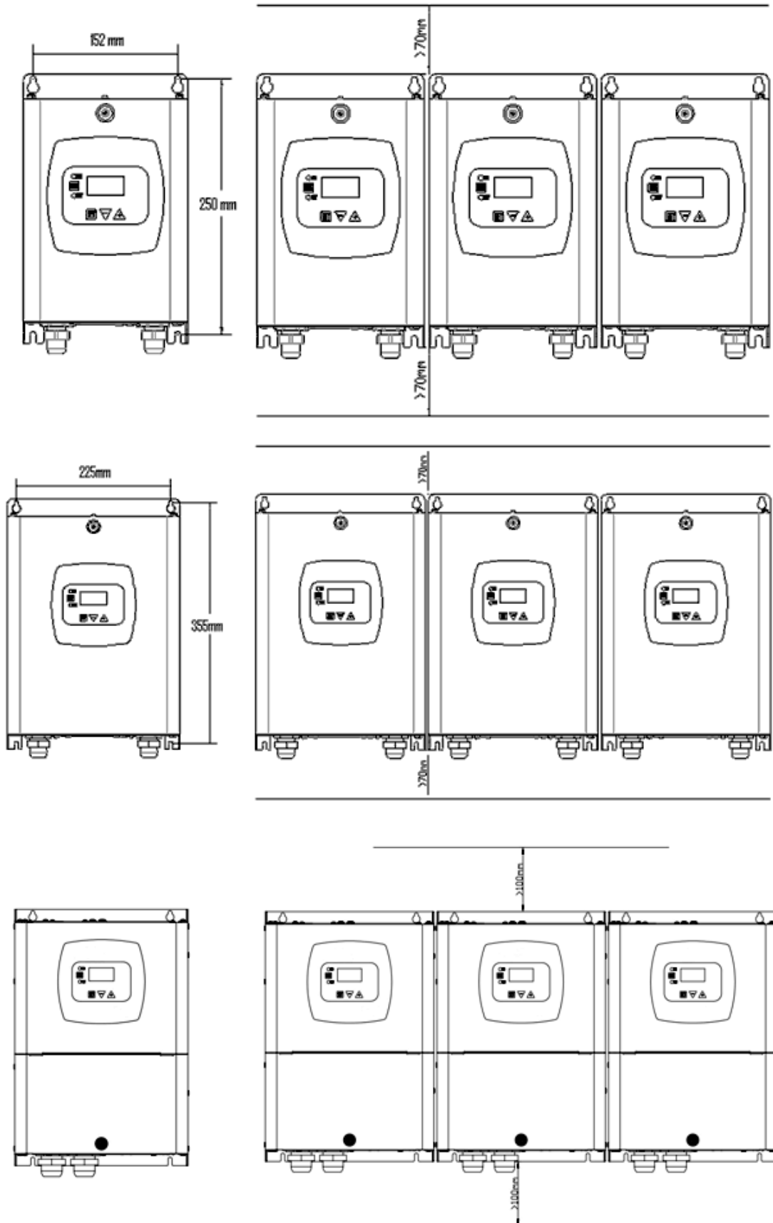
Figure 2: Fixture and minimum clearance for air circulation
