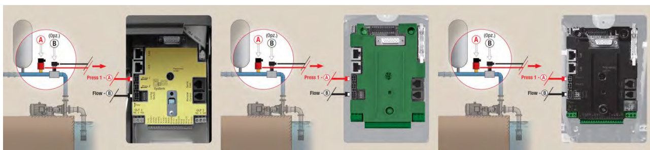
Figure 7: Sensor connections
