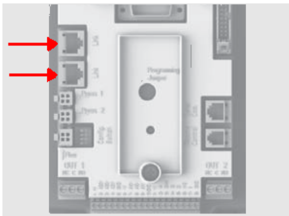
Figure 16: Link connection
