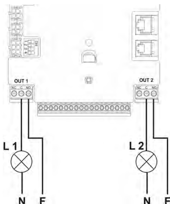
Figure 10: Example of output connections
