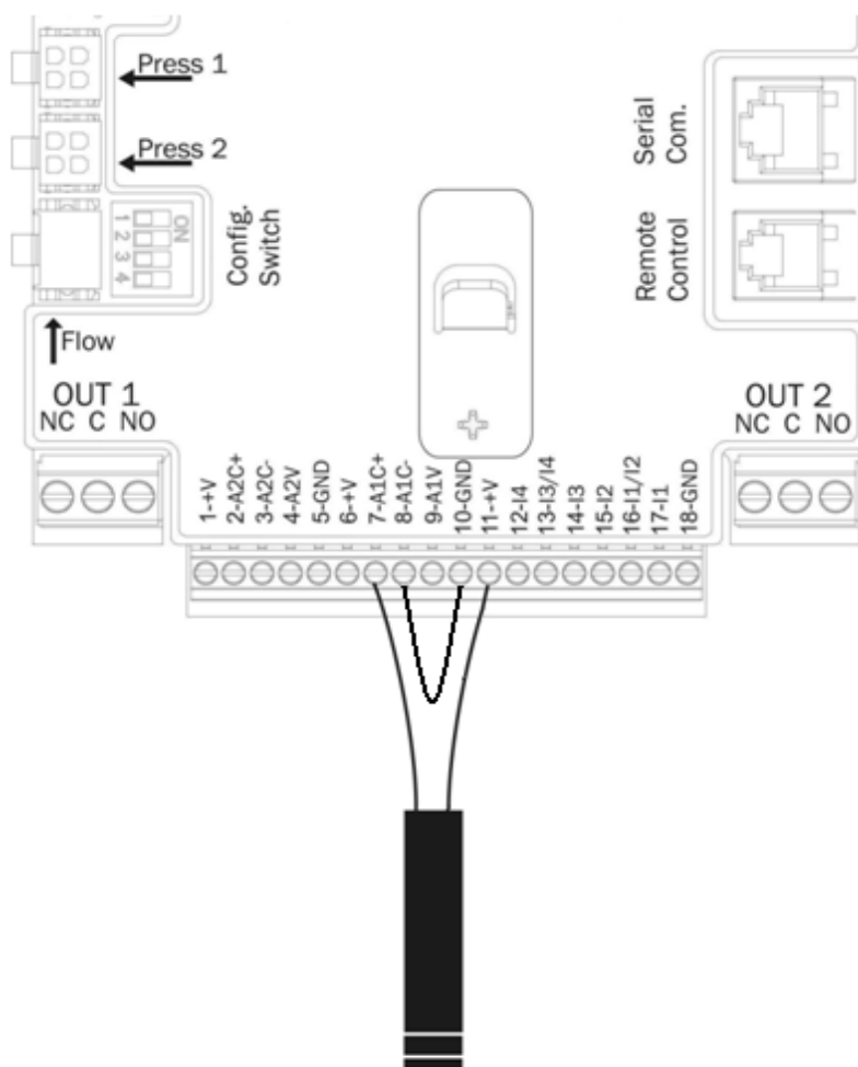
Figure 8: Connecting the 4 - 20 mA pressure sensor
