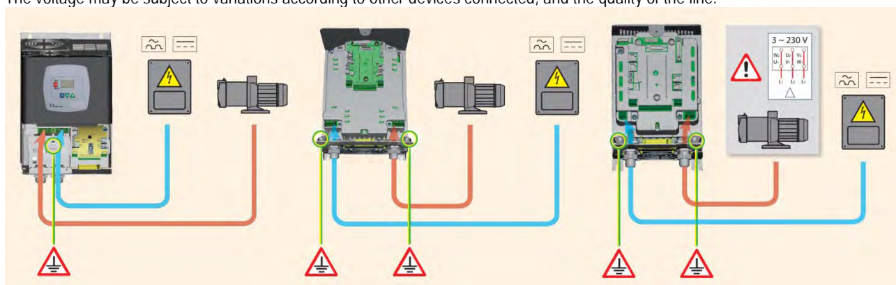
Figure 4: Electrical connections
