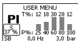
Figure 13: Power histogram
