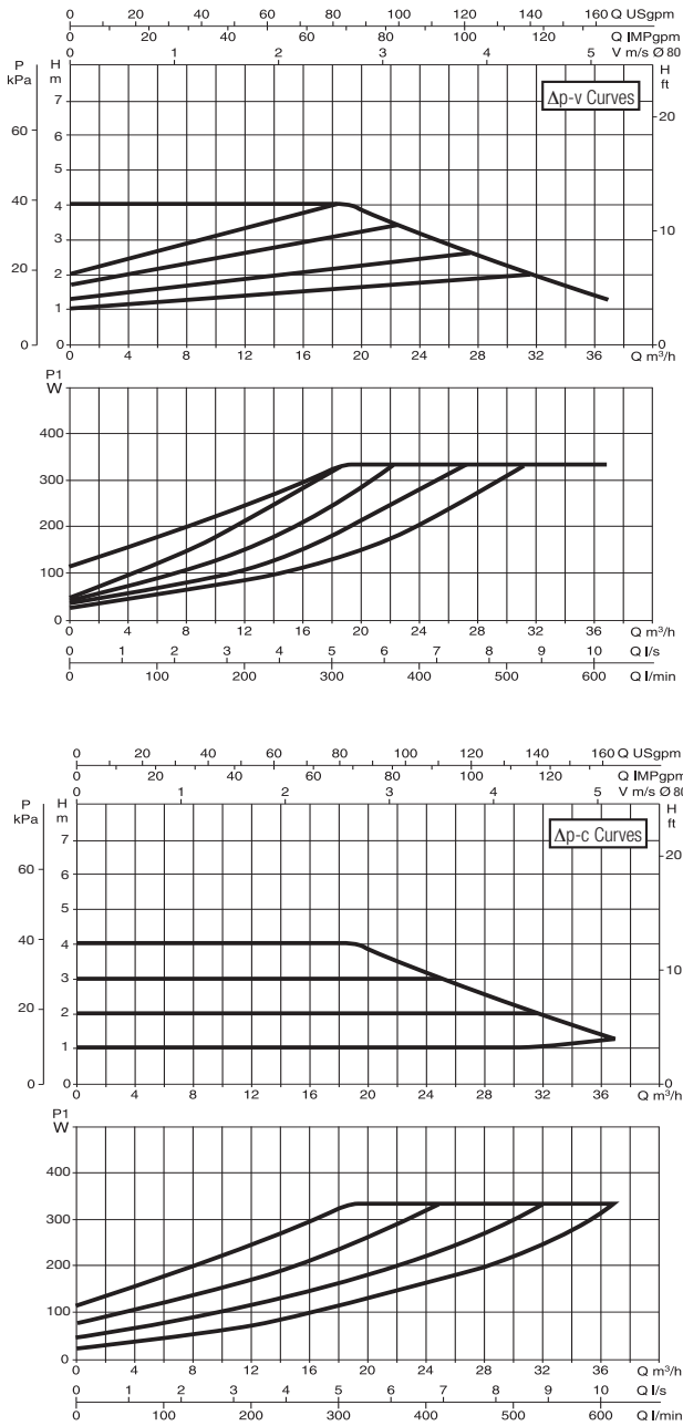
EVOPLUS B 40/360.80 M
