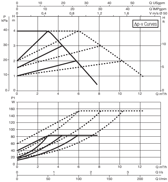
EVOPLUS D 40/220.32 M
