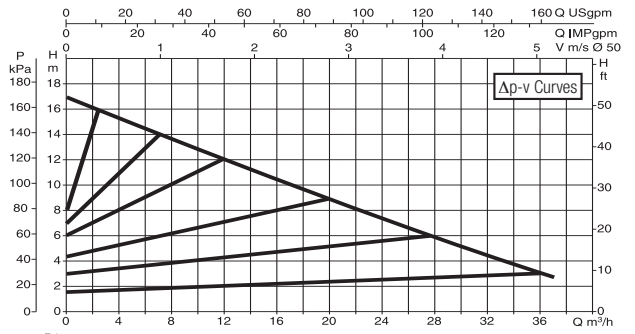
EVOPLUS B 180/280.50 M
