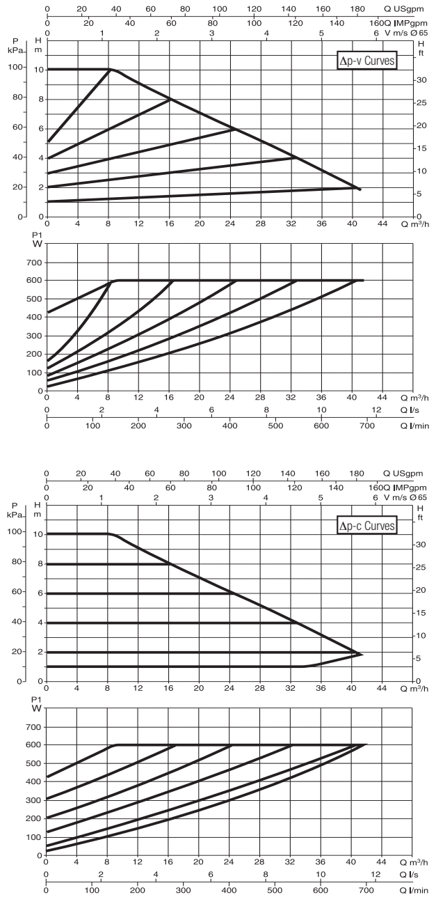
EVOPLUS B 100/340.65 M
