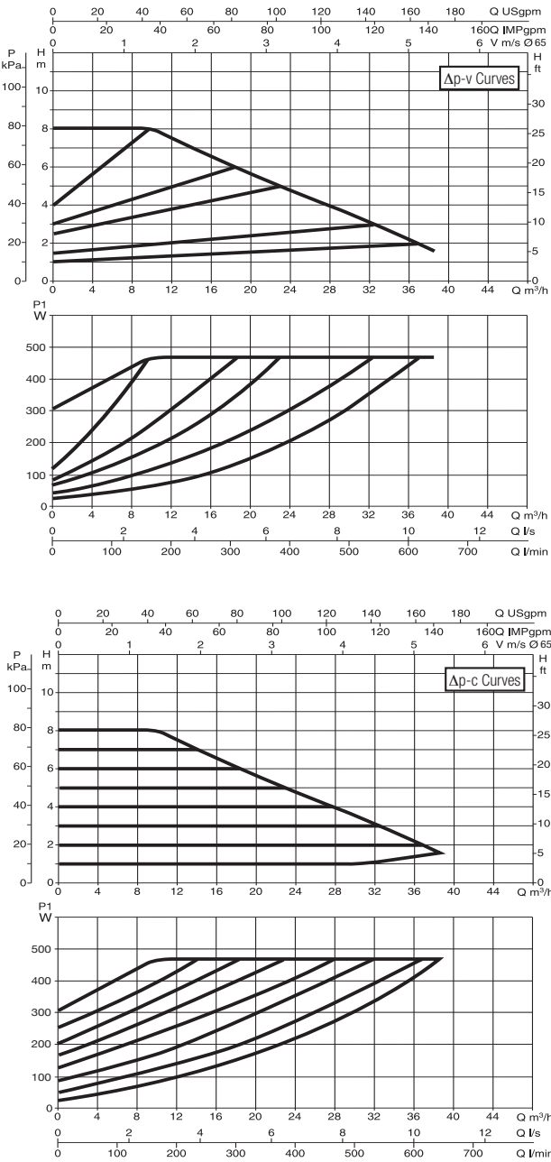
EVOPLUS B 80/340.65 M
