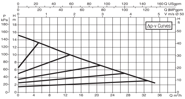
EVOPLUS B 150/280.50 M
